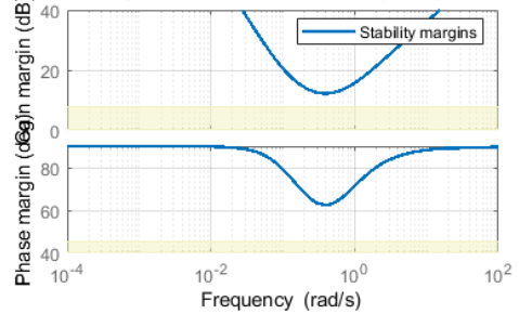
Margins at plant inputs: Stability margins
