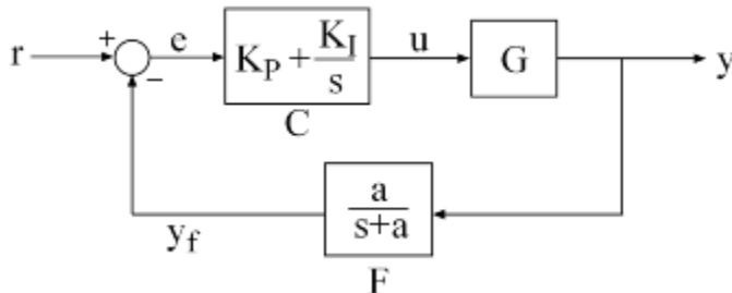
Figure 1: Control Structure
