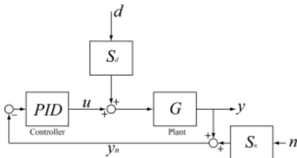
Figure 2: Regulation loop.
