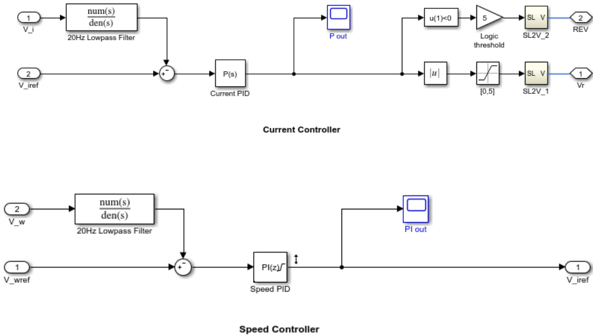
Figure 1: Current and Speed Controllers.
