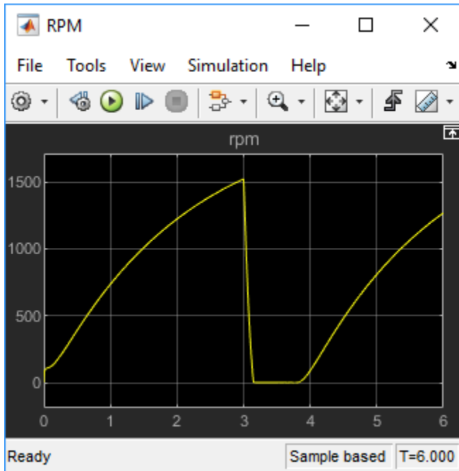
Figure 2: Untuned Response.
